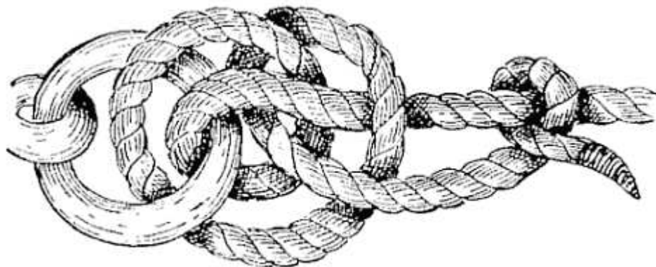
FIG. 53.—Fisherman's hitch.
