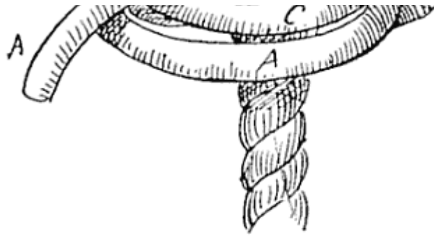
FIG. 132.—Matthew Walker (complete but slack).
