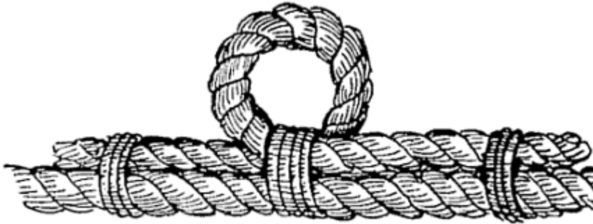
FIG. 96.—Lashed cut-splice.
