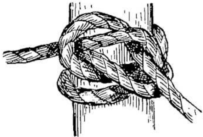
FIG. 27 —Gunner's knot.
