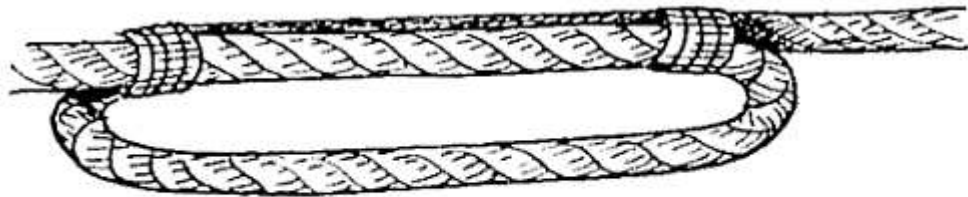
FIG. 76.—Seized shortening.
