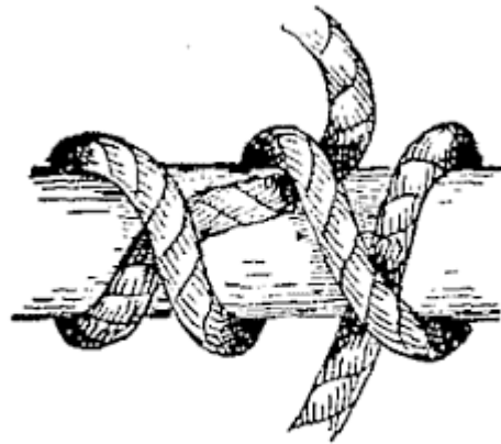
FIG. 48.—Rolling hitch.
